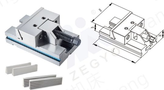
ZQ84-I 动钳组件 MOVABLE JAW SECTION
